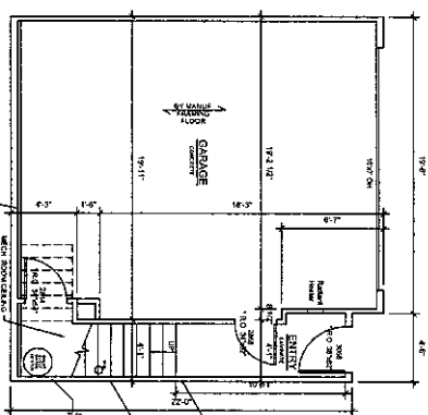
4 Garage Plan, Mirrored SCALE: 1/8"=1'-0"
