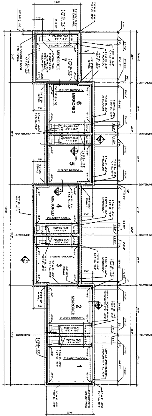
1 Foundation Plan SCALE 1/8"=1'-0"
