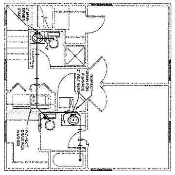
3 Upper Level Plan SCALE: 1/8"=1'-0"
