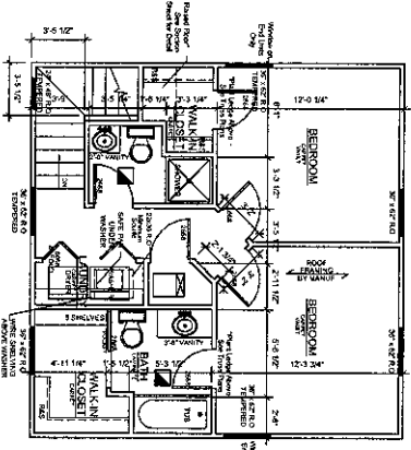
3 Upper Level Plan SCALE: 1/8"=1'-0"
