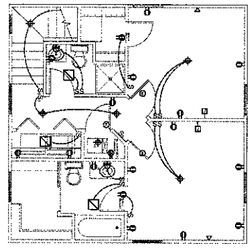
3 Upper Level Plan SCALE 1/4"=1'-0"
