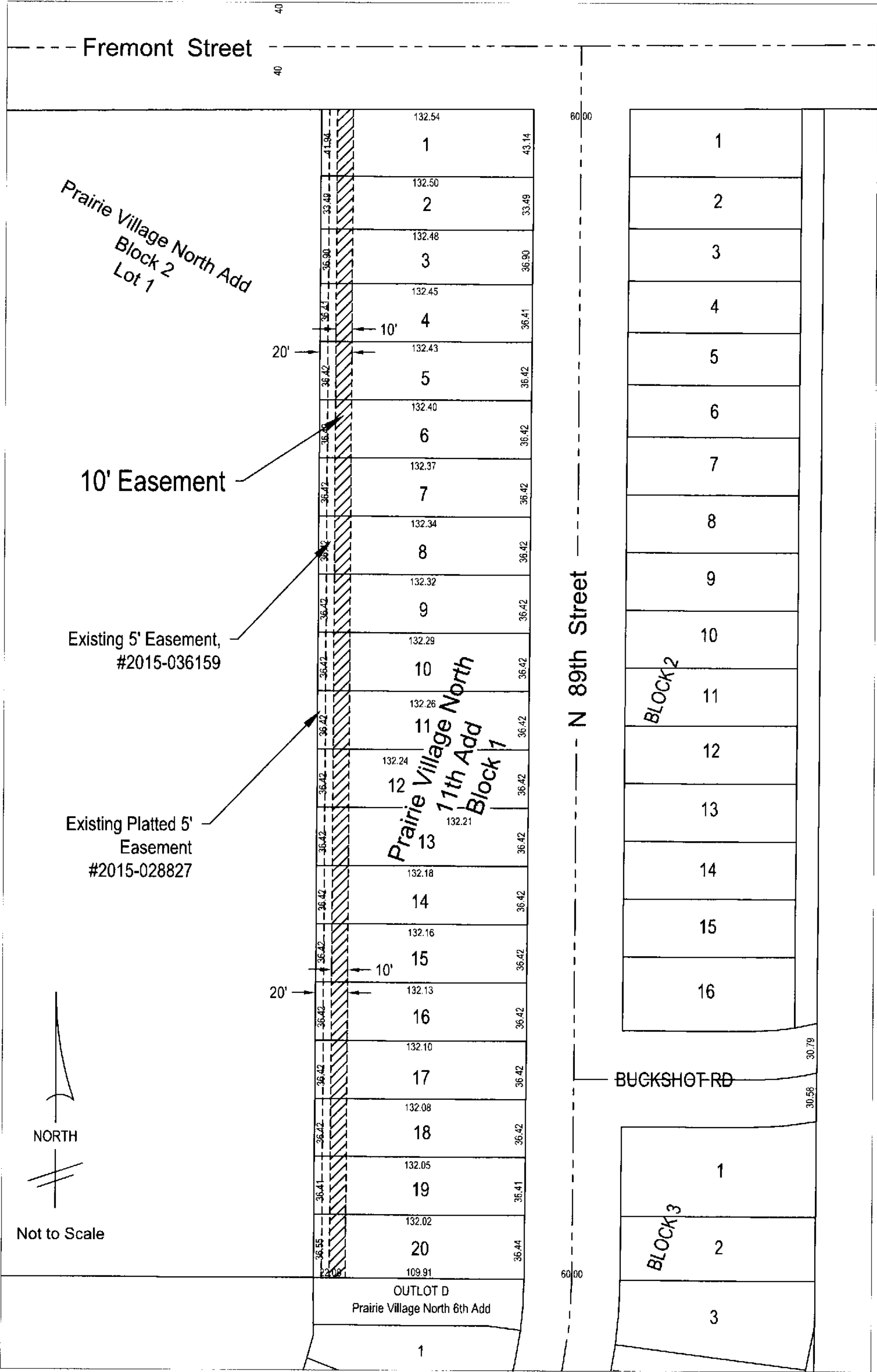
Location of a Utility Easement lying within Lots 1-20, Block 1, Prairie Village North 11th Addition, in the SW 1/4, Section 11, Township 10 North, Range 7 East of the 6th P.M., Lincoln, Lancaster County, Nebraska.
