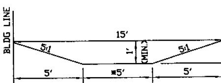
TYPICAL SWALE SECTION
