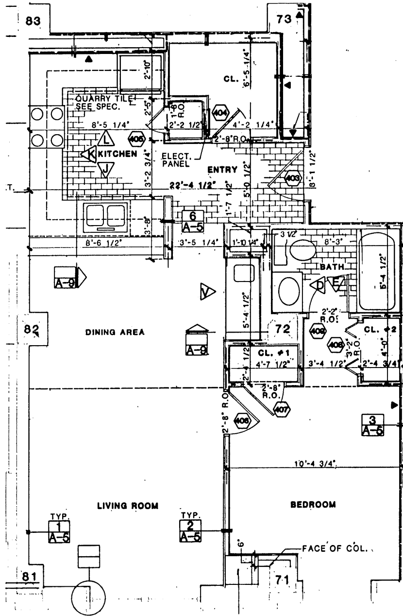
PLAN TYPE H (616.96 S.F.)
