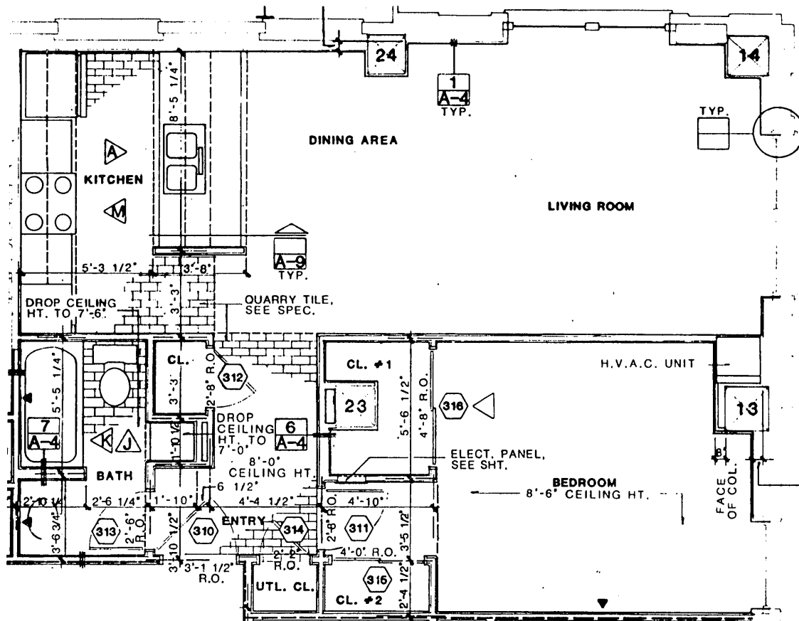
PLAN TYPE G (639.84 S.F.)
