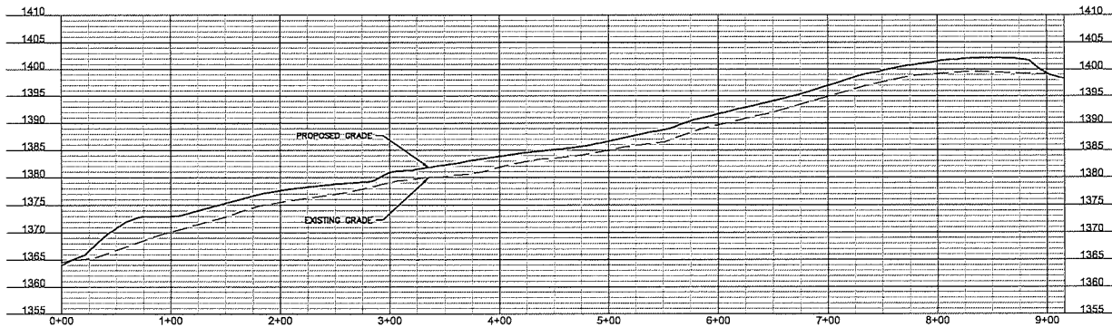
NNG ALIGNMENT (0+00 - 9+15.84)
