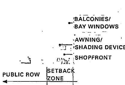
Commercial Setback Diagram
