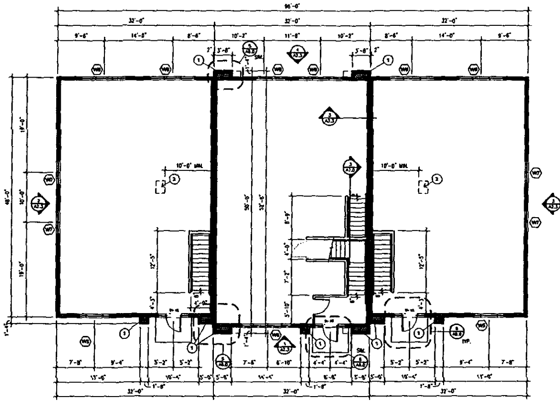
1 FIRST FLOOR PLAN - BUILDING B
