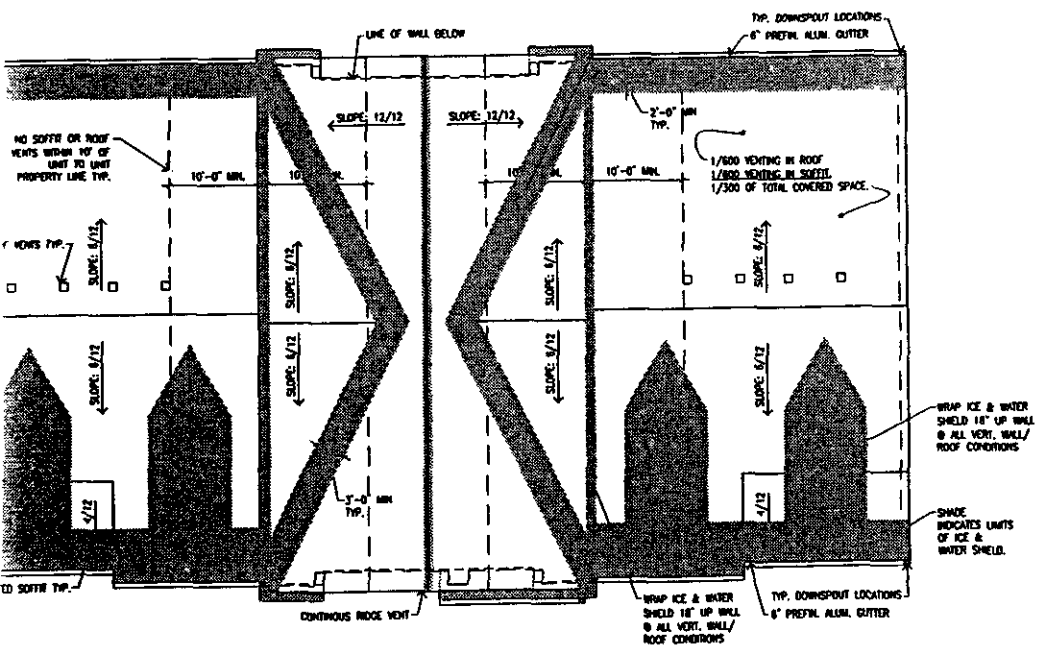
ROOF PLAN - BUILDING B
