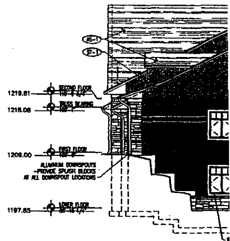
3 SIDE ELEVATION - BUILDING B A23 1/8" = 1'-0"
