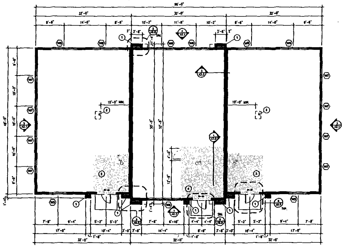
1 FIRST FLOOR PLAN - BUILDING A A2.0 1/8" = 1'-0"
