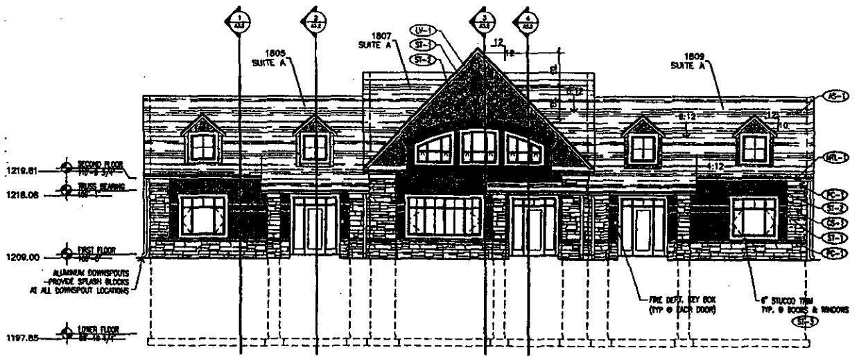
1 FRONT ELEVATION - BUILDING B A23 1/8" = 1'-0"
