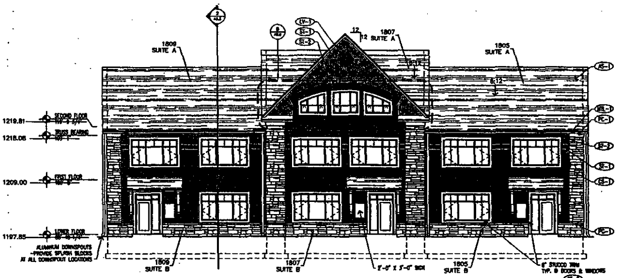
4 REAR ELEVATION - BUILDING B A23 1/8" = 1'-0"
