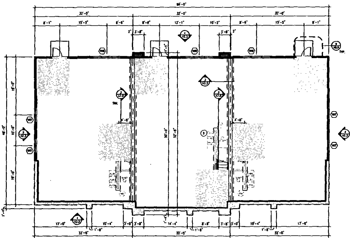
3 BASEMENT PLAN - BUILDING B
