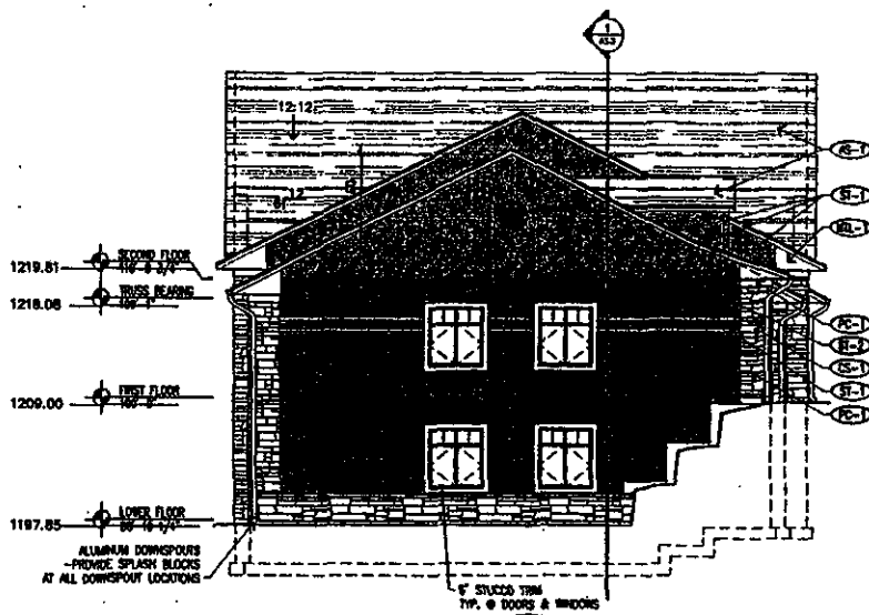
2 SIDE ELEVATION - BUILDING B A23 1/8" = 1'-0"
