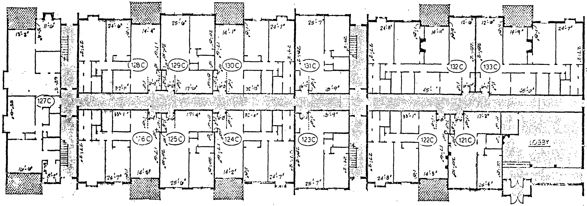
FIRST FLOOR WING "C"
