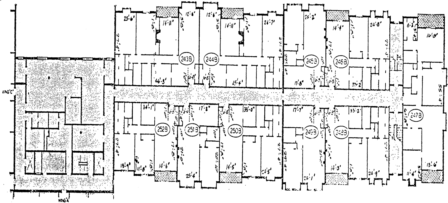
SECOND FLOOR WING "B"
