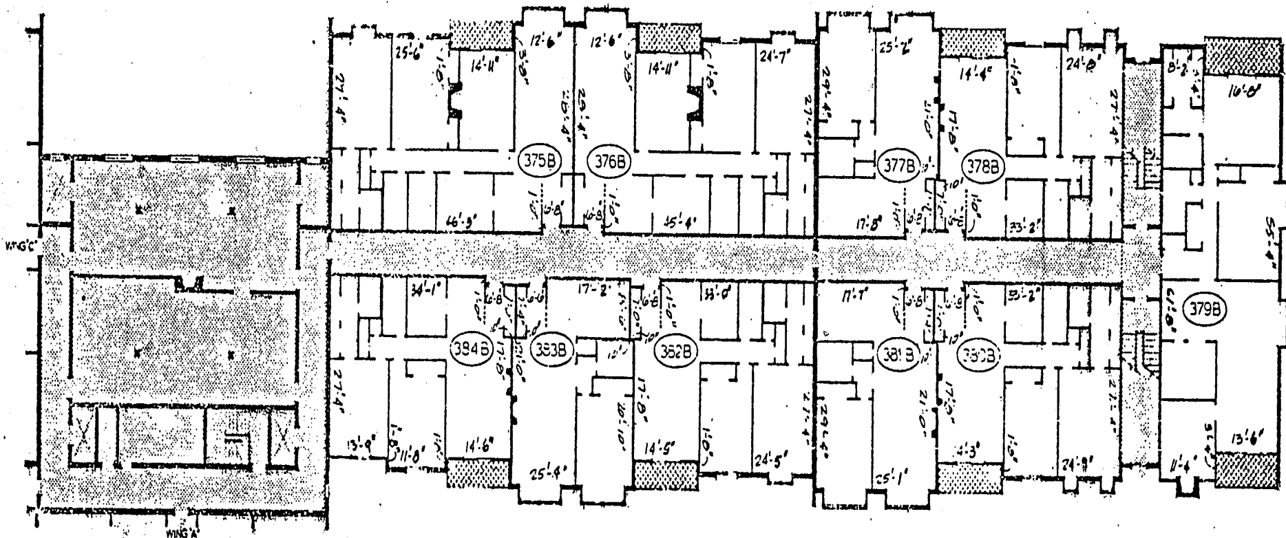
THIRD FLOOR WING "B"
