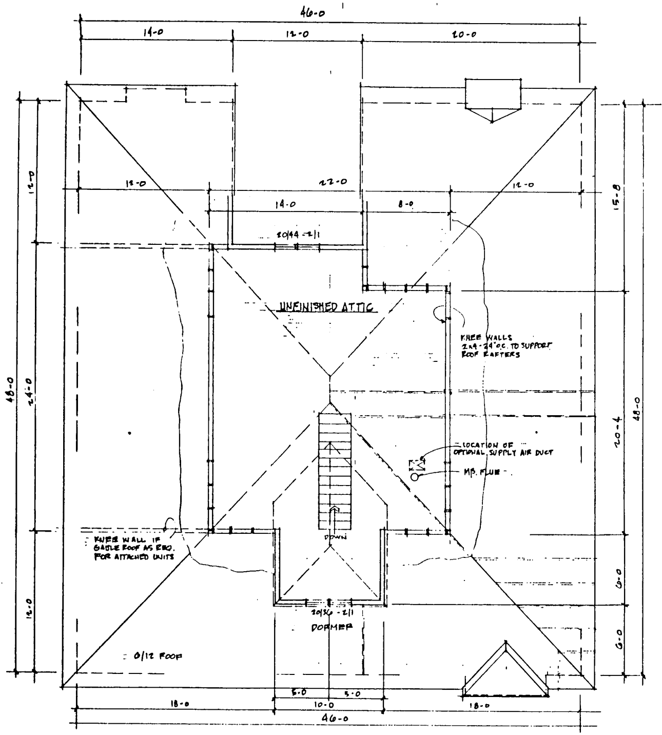
ATTIC FLOOR PLAN 1/4" = 1'-0"
