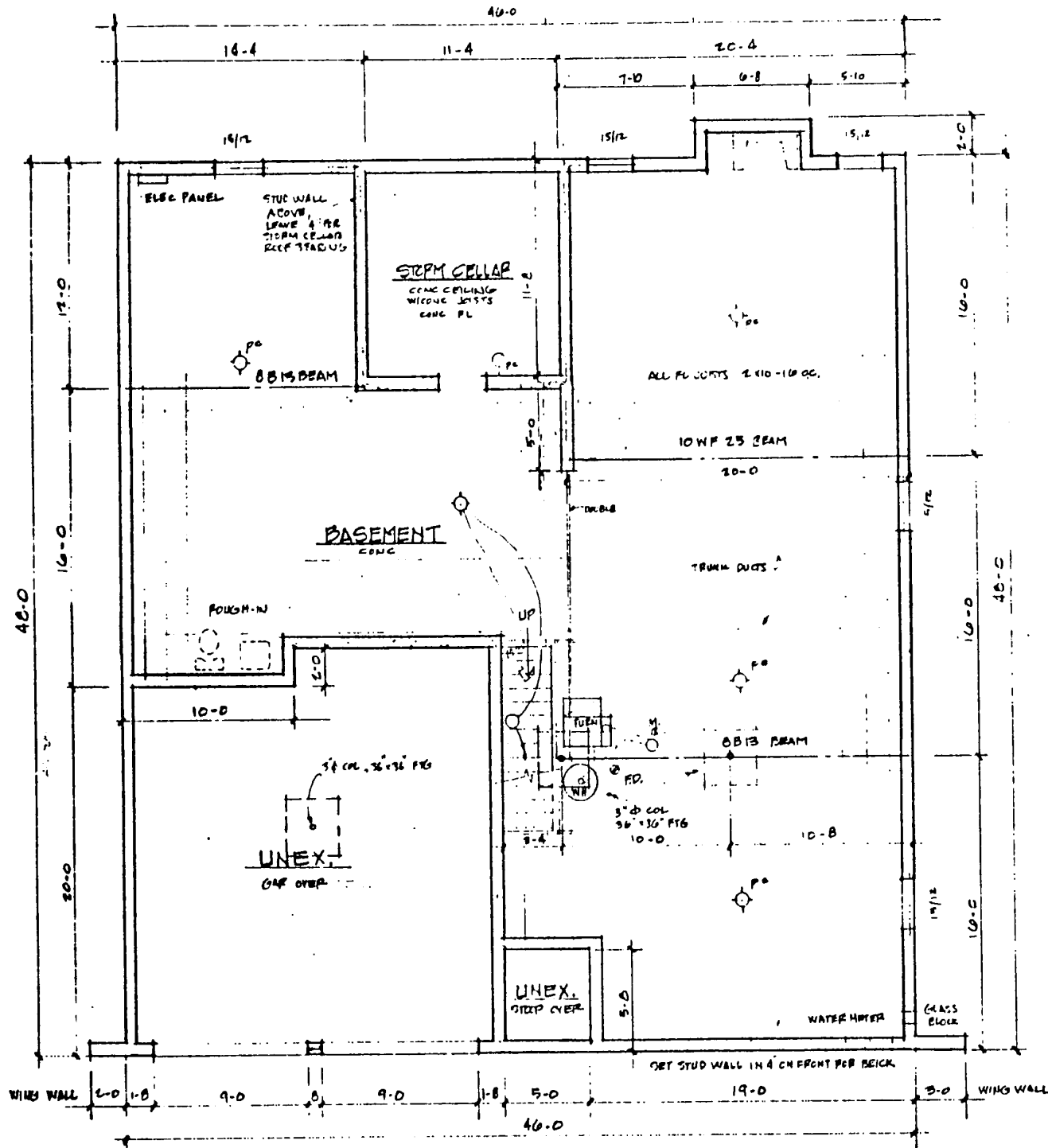
BASEMENT PLAN
