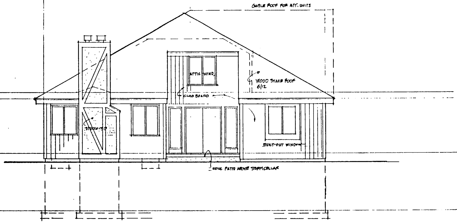
REAR ELEVATION 1/4" = 1'-0"
