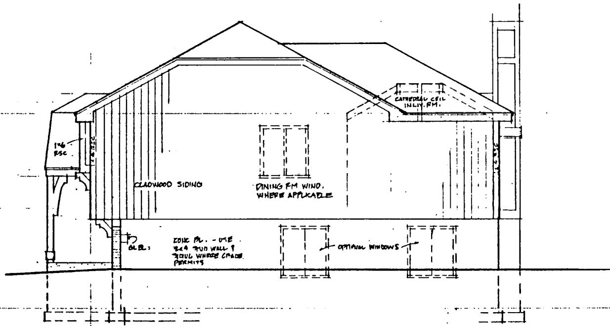
RIGHT ELEVATION 114'-11\"/>
