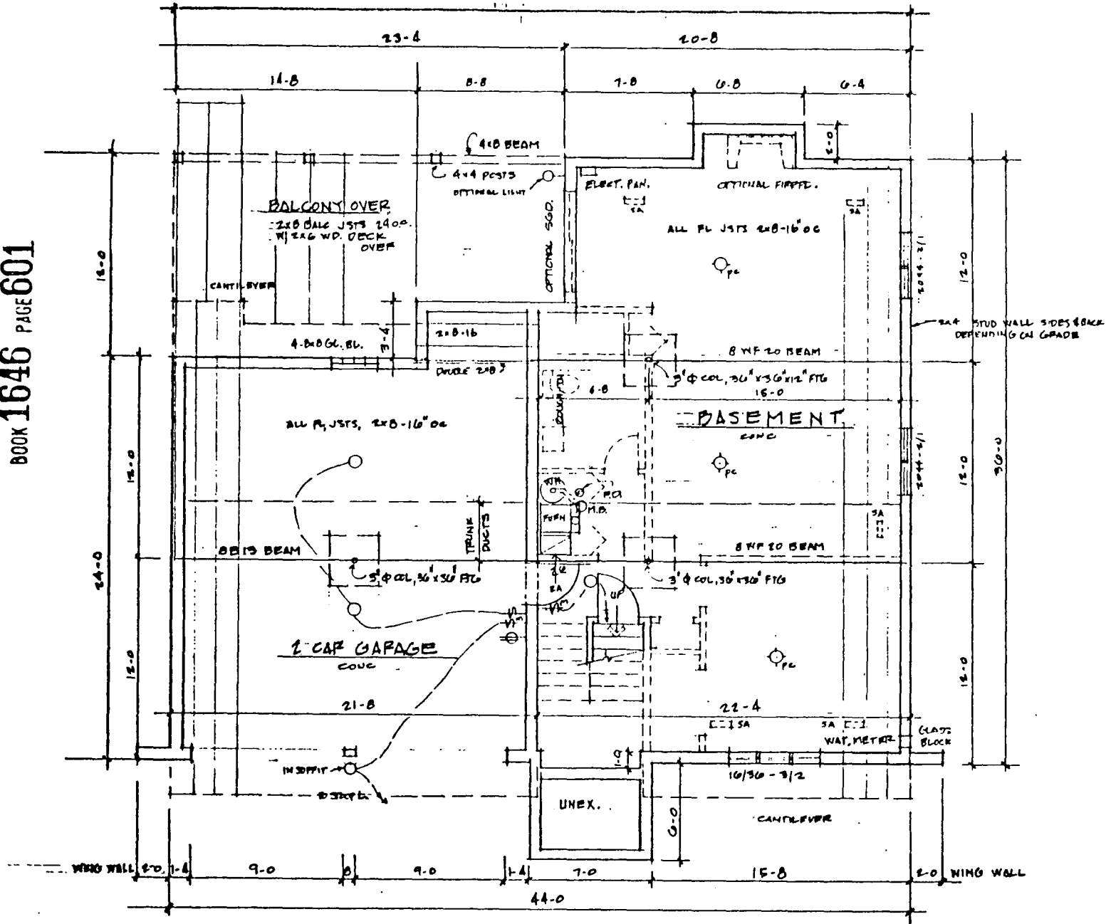
BASEMENT PLAN (UNFIN. BSMT) scale 1/4" = 1'-0"
