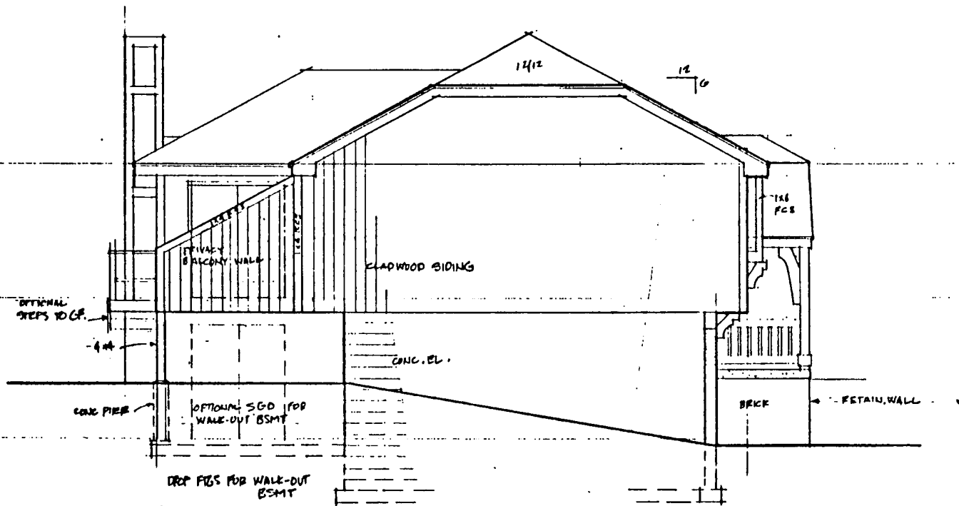
LEFT ELEVATION 114'-11\"/>
