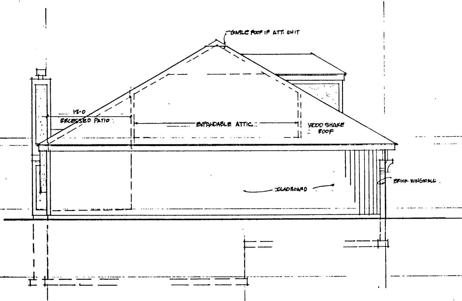
LEFT ELEVATION 14'-10"
