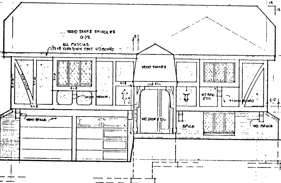
FRONT ELEVATION "A" 1/4" = 1'-0"
