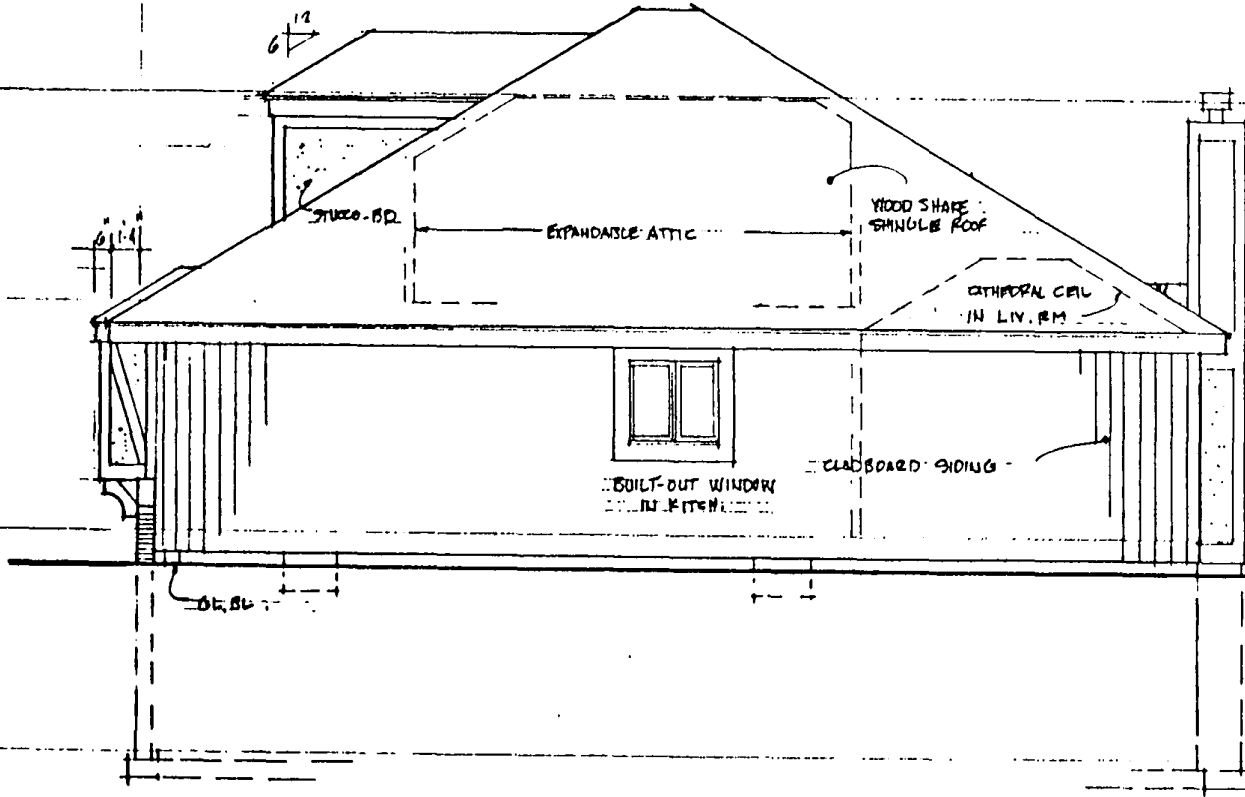
RIGHT ELEVATION 1/4"=1'-0"
