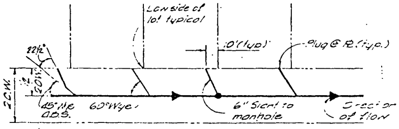
TYPICAL NYE OR SLANT DETAIL
