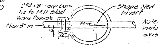
CONNECTION TO EXIST MANHOLE DETAIL
