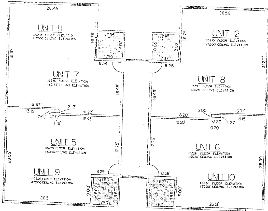
SECOND & THIRD FLOOR PLAN
