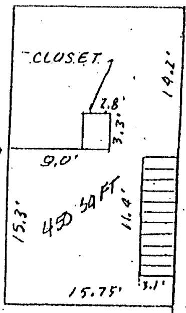
MAIN FLOOR TYPE A
