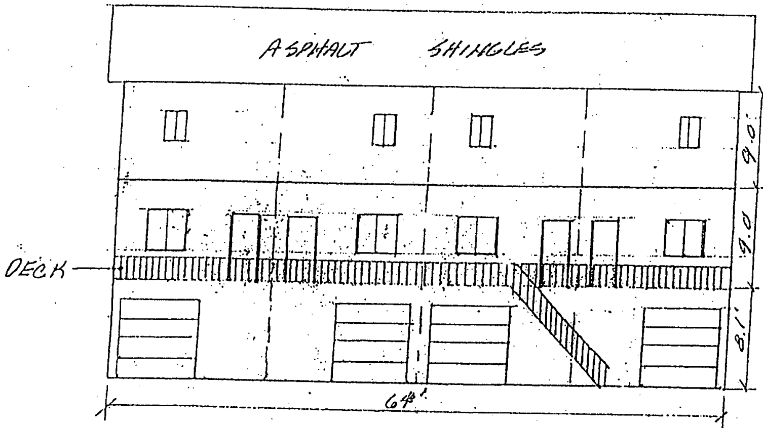
FRONT ELEVATION 4 UNIT
