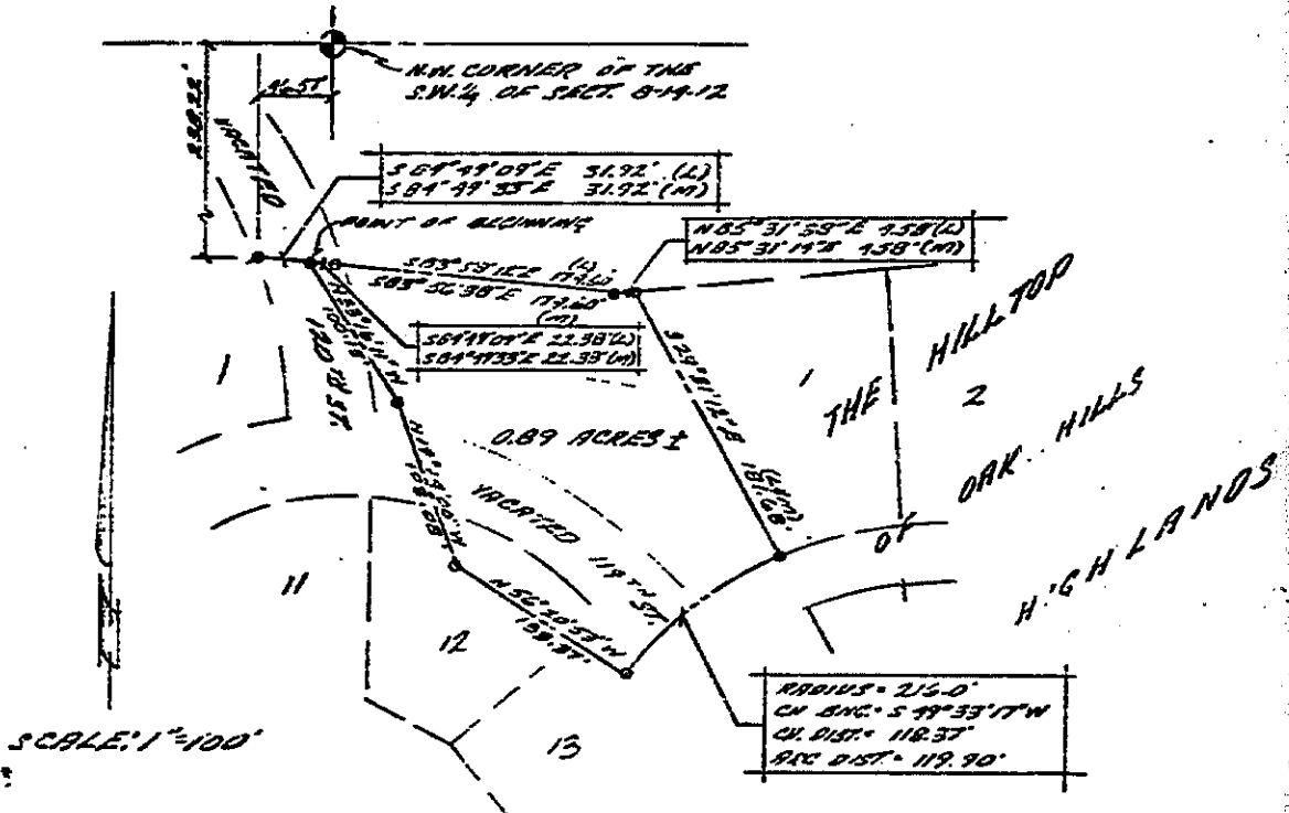
Plot to scale showing tract surveyed with all pertinent points.
