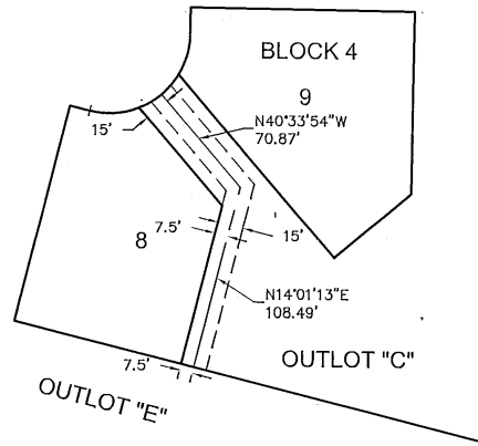
PEDESTRIAN EASEMENT DETAIL SCALE: 1" = 80'
