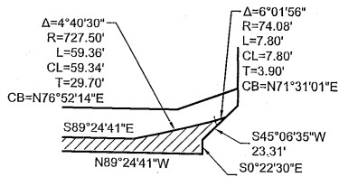
"A" STREET ROW DEDICATION DETAIL SCALE: 1" = 80'
