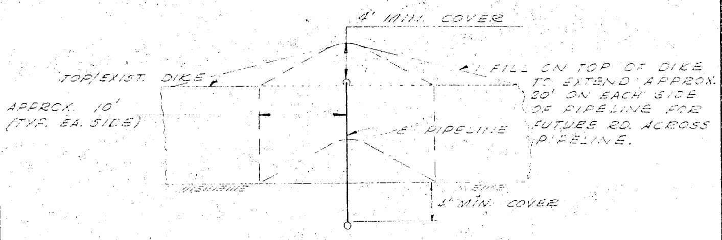
SECTION A
