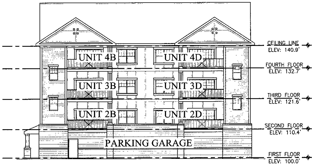
WEST ELEVATION
