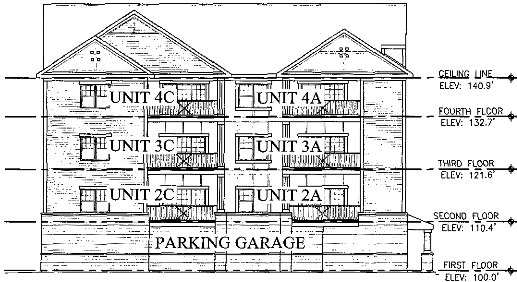
EAST ELEVATION
