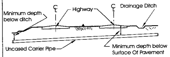
UNCASED HIGHWAY CROSSING FIGURE 4
