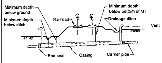
CASED RAILROAD CROSSING FIGURE 1
