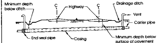
CASED HIGHWAY CROSSING FIGURE 2
