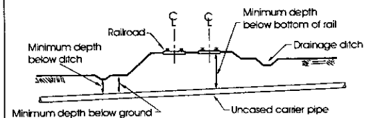
UNCASED RAILROAD CROSSING FIGURE 3
