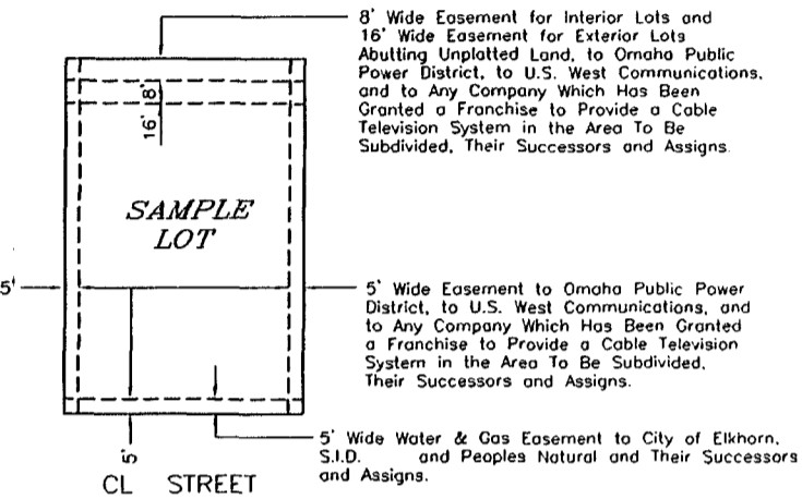
TYPICAL LOT DEDICATION EASEMENTS
