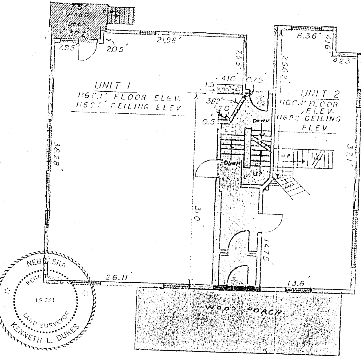
FIRST FLOOR PLAN NO SCALE
