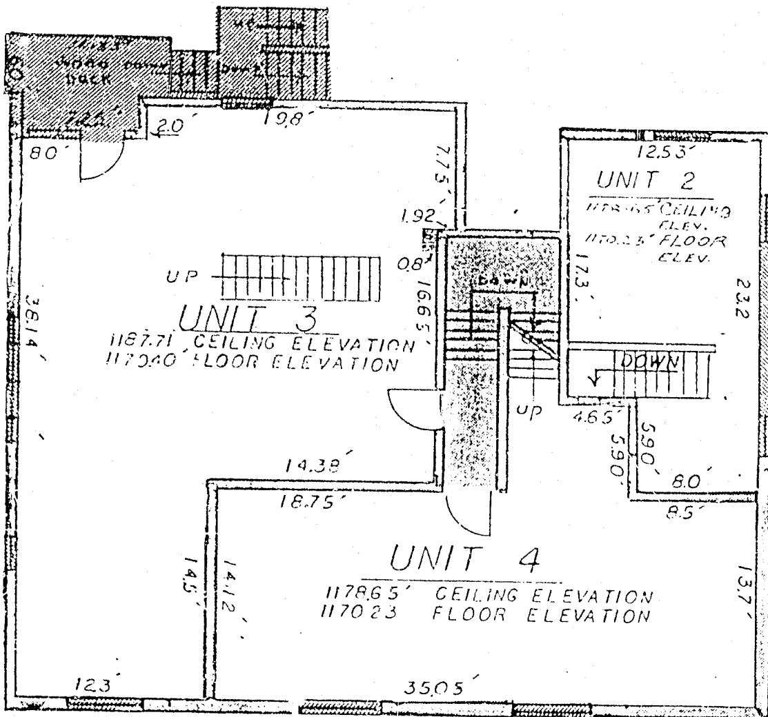
SECOND FLOOR PLAN NO SCALE
