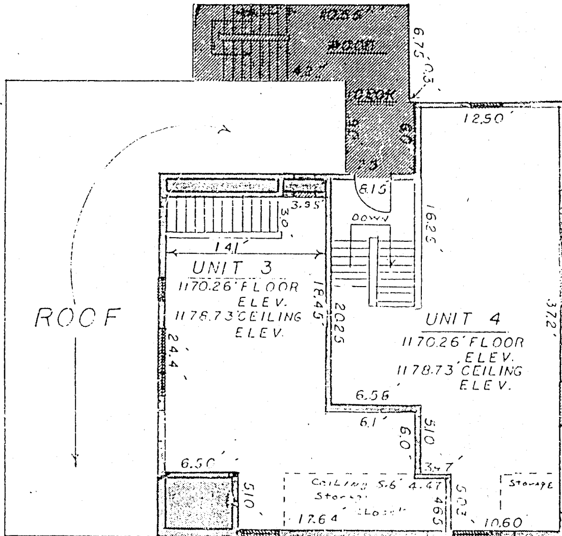
THIRD FLOOR PLAN NO SCALE
