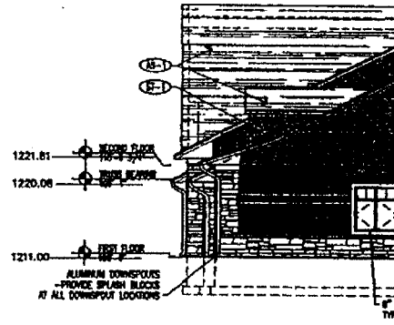
3 SIDE ELEVATION - BUILDING A A21 1/8" = 1'-0"
