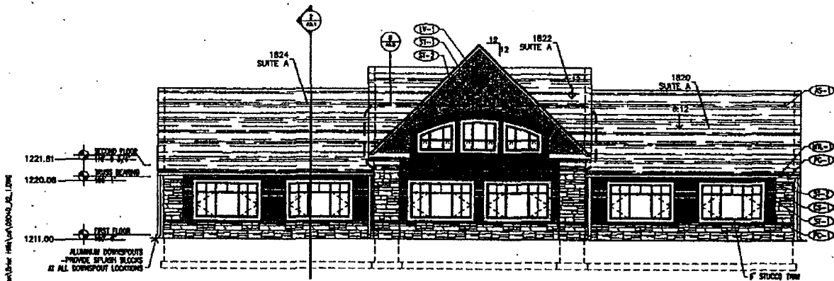
4 REAR ELEVATION - BUILDING A A21 1/8" = 1'-0"
