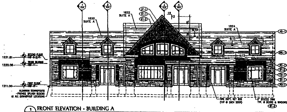
1 FRONT ELEVATION - BUILDING A A21 1/8" = 1'-0"
