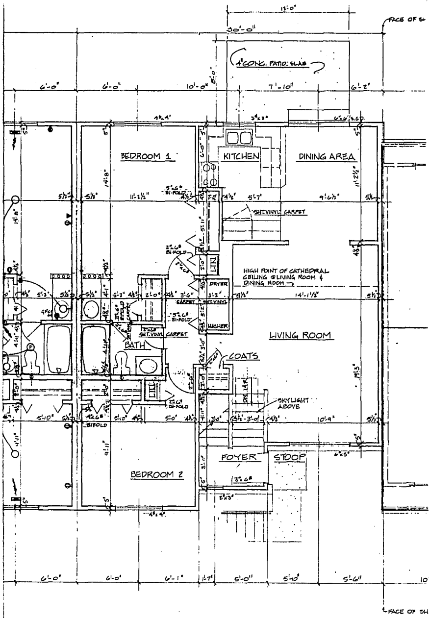
UPPER LEVEL PLAN SCALE 1/4" = 1'-0"
