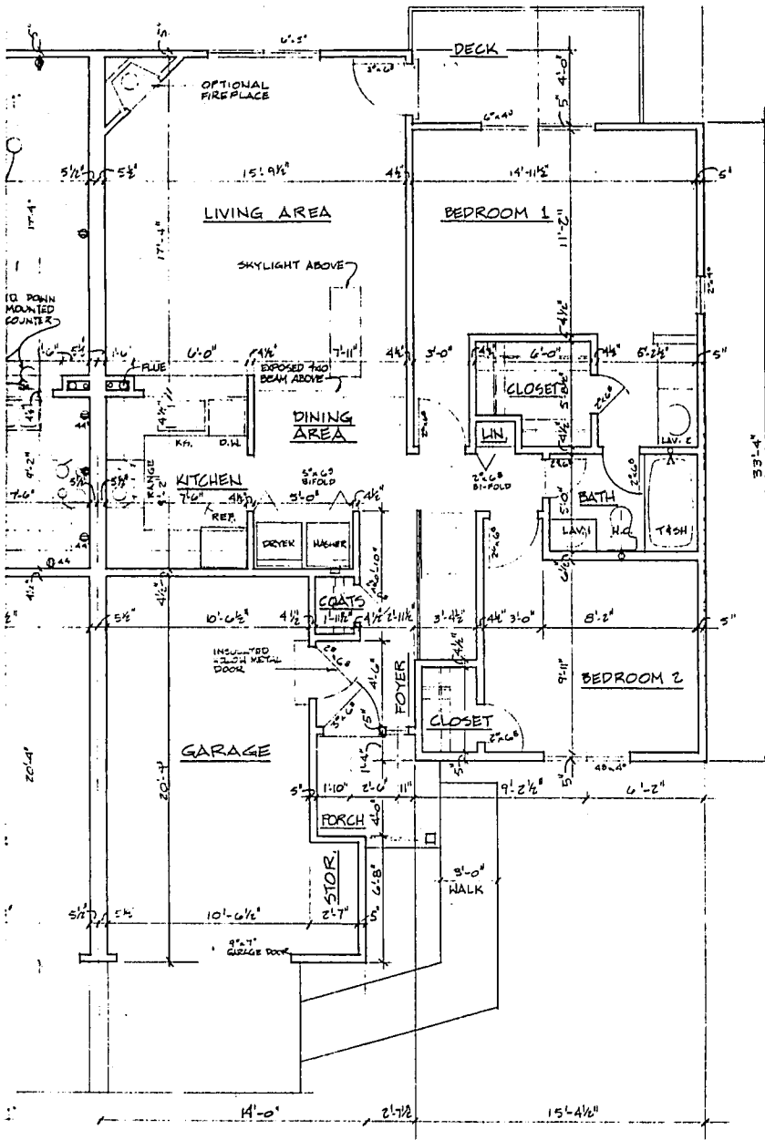
UPPER LEVEL PLAN SCALE 1/4" = 1'-0"
