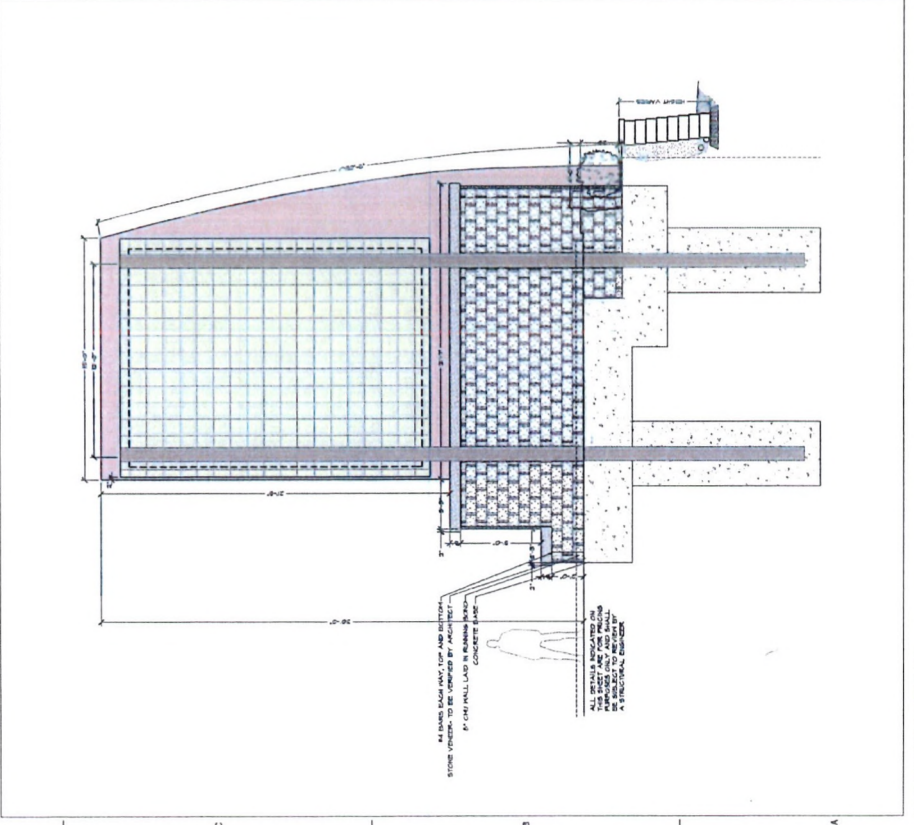
7 MONUMENT SIGN SCALE: 1/4" = 4'-0" SECTION
